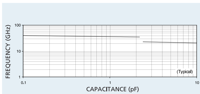
Fig. 1 Typical first parallel resonant frequency.
