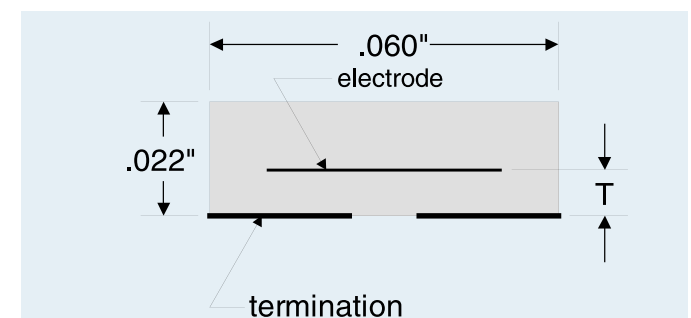
Fig. 2 Typical longitudinal cross section.
